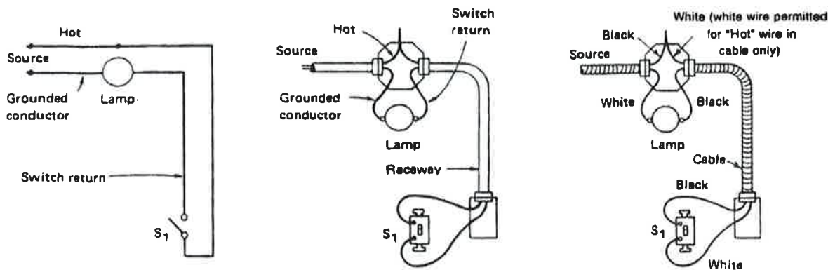
(B) Circuit with single-pole switch feed at light
